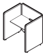
Without Return Panel (Without Screen) L 1200 x W 950 x H 1200 mm
