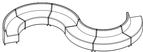
S Shape 6 Piece L 5140 x D 4625 x H 750 m
