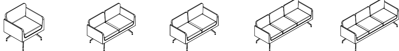
Single Seater L 700 x D 665 x H 780 Two Seater L 1200 x D 665 x H 780 Two & Half Seater L 1500 x D 665 x H 780 Three Seater L 1800 x D 665 x H 780 Three & Half Seater L 2100 x D 665 x H 780
