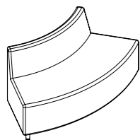
Convex Outer R 1650 / Inner R 1000 x D 650 x H 750 mm
