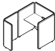
With Return Panel (Without Screen) L 1200 x W 1800 x H 1200 mm
