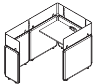
With Return Panel (With Screen) L 1200 x W 1800 x H 1200 mm
