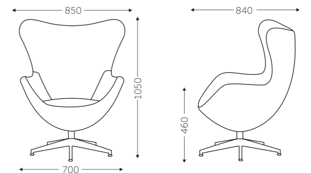
Aluminium Base
